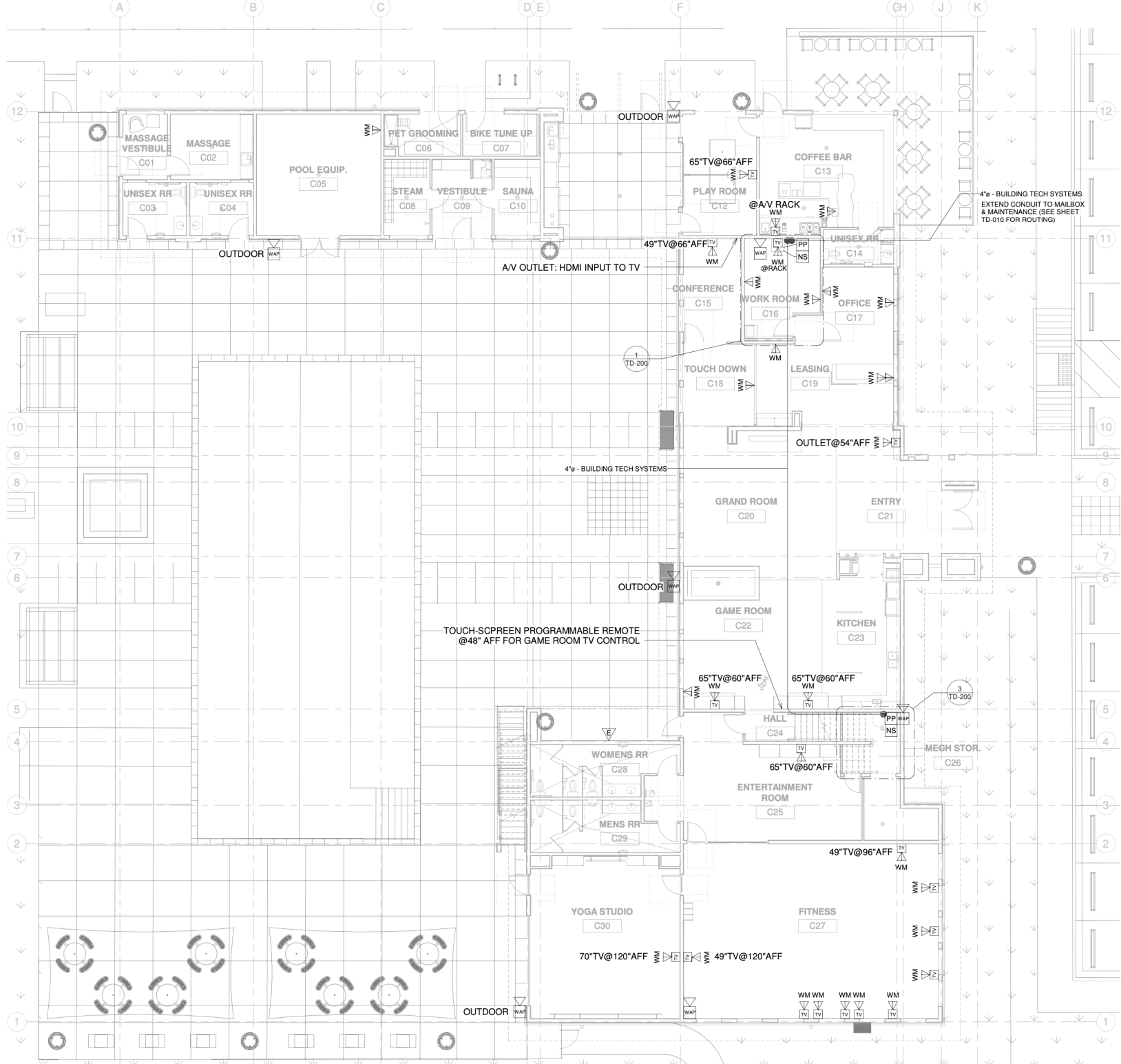
LEVEL 1 - DATACOMM LAYOUT
