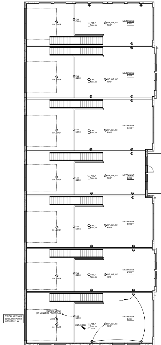
MEZZANINE LEVEL POWER PLAN SCALE: 1/8"=1'-0"
