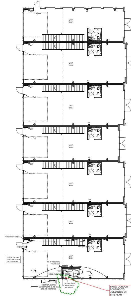
GROUND LEVEL POWER PLAN SCALE: 1/8"=1'-0"
