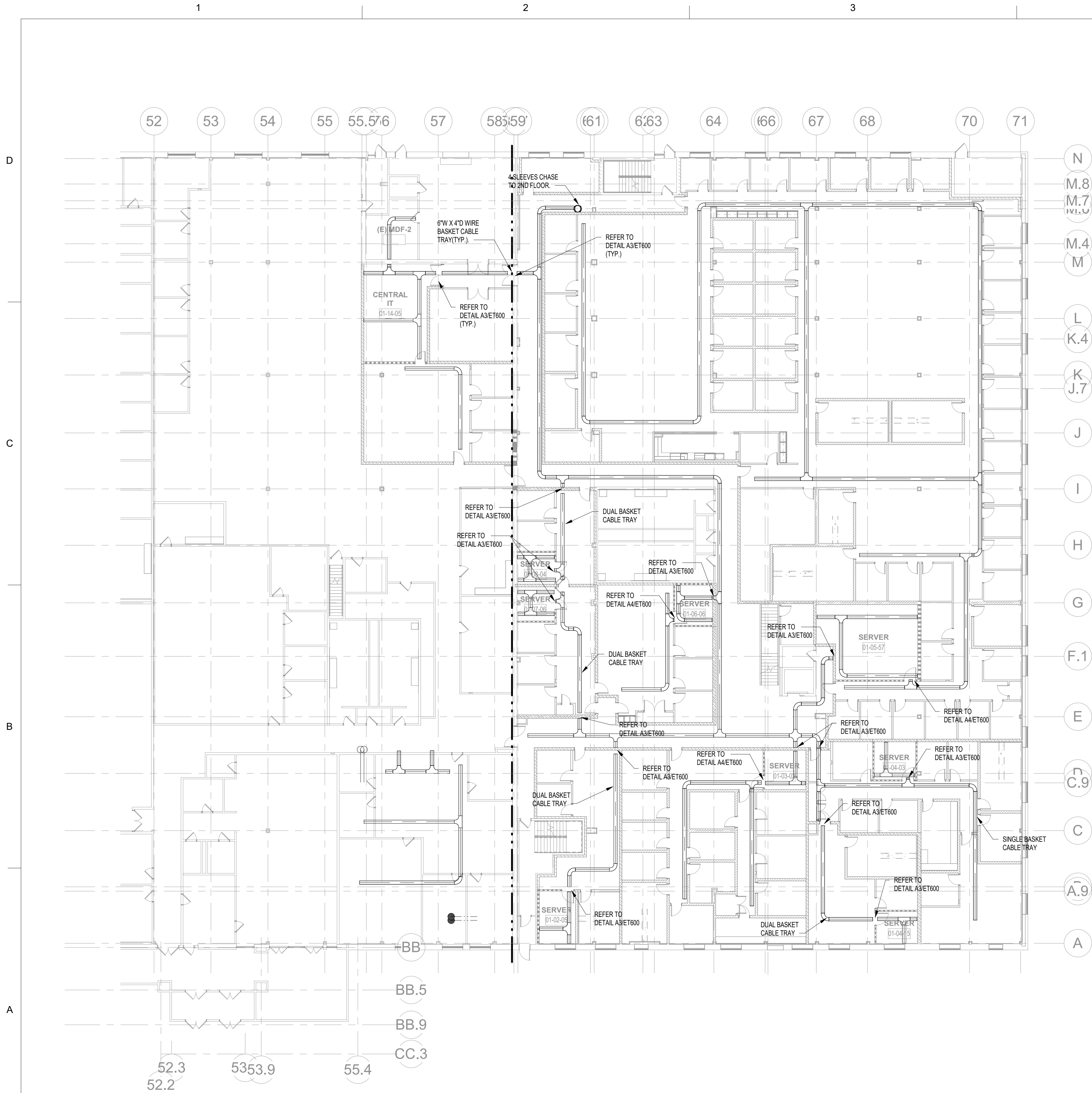
A1 1ST FLOOR TELECOMMUNICATIONS OVERALL CABLE TRAY PLAN SCALE: 1/16" = 1'-0"
