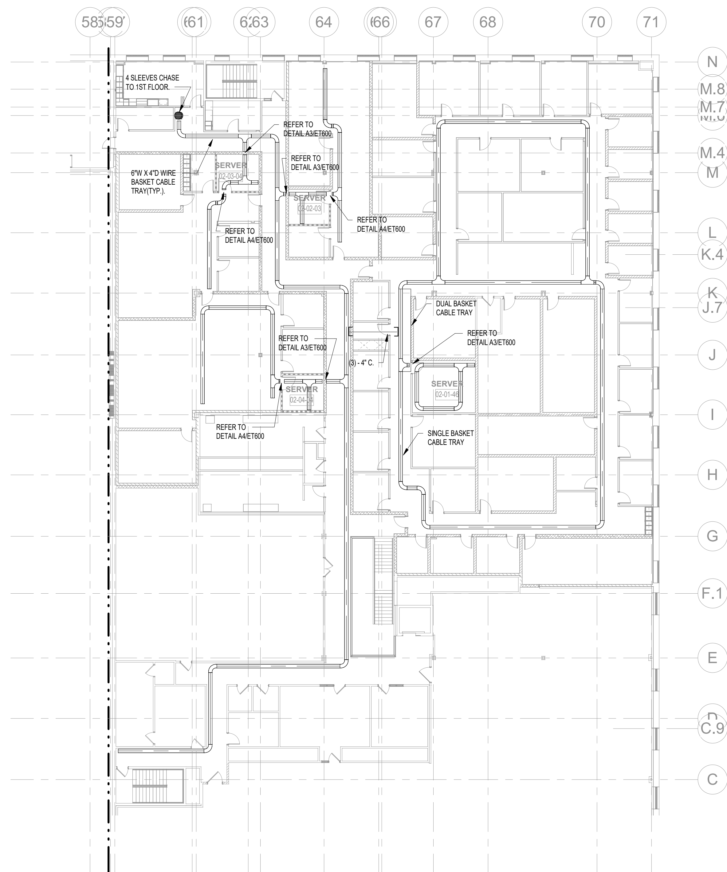
A1 2ND FLOOR TELECOMMUNICATIONS OVERALL CABLE TRAY PLAN SCALE: 1/16" = 1'-0"
