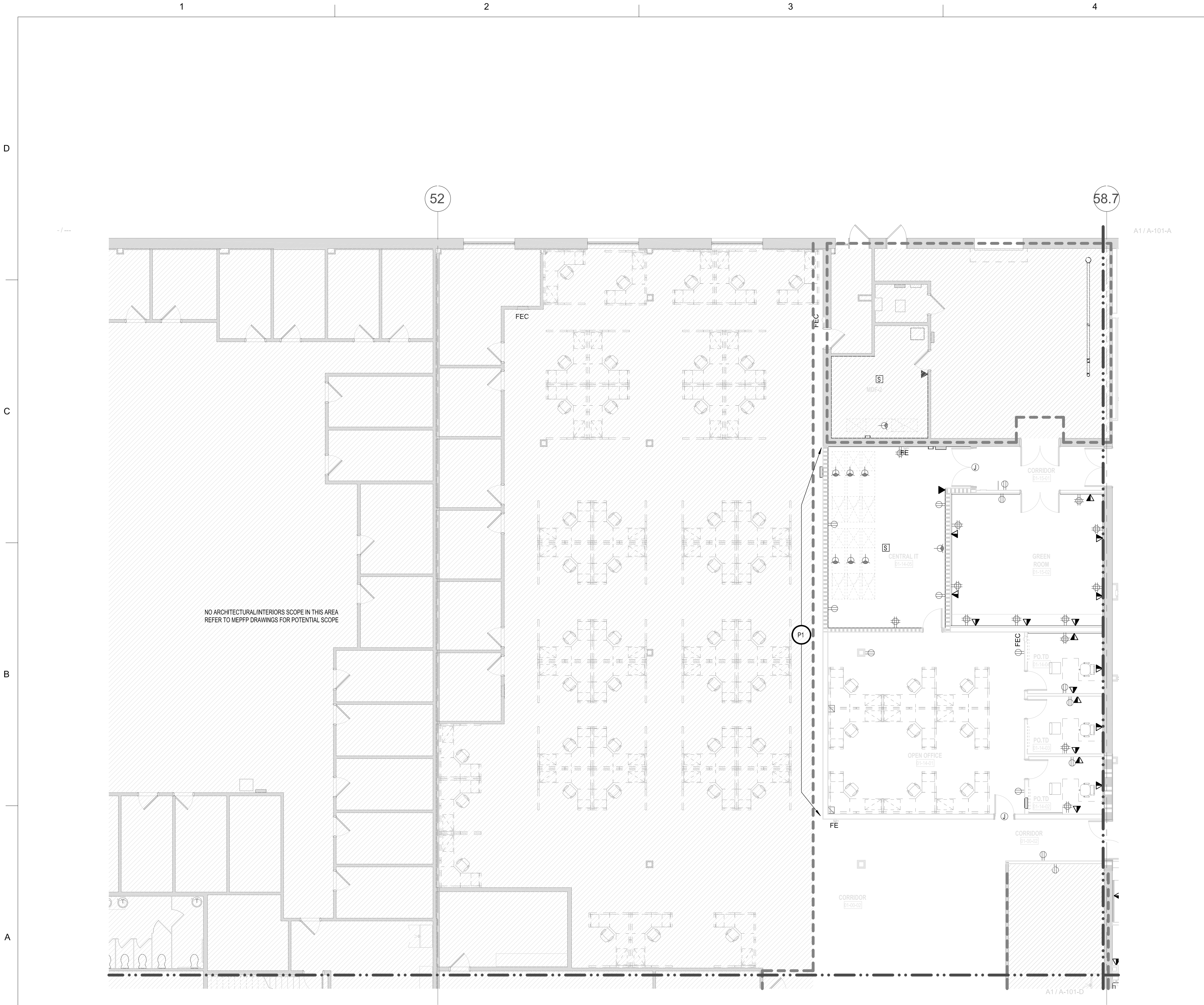
A1 1ST FLOOR TEL/DATA PLAN - PART C SCALE: 1/8" = 1'-0"
